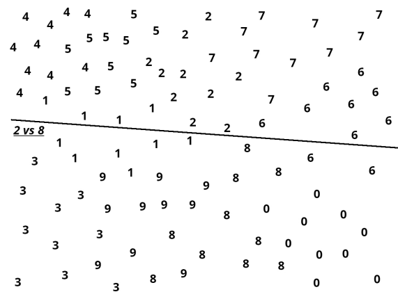
Fig. 1. One-versus-one approach.
