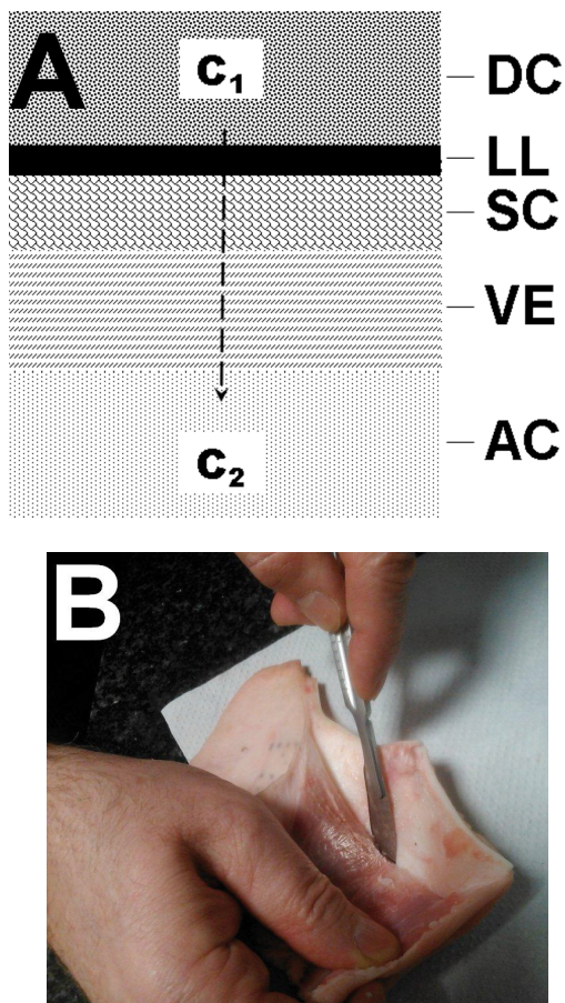
Figure 5. Visualization of the skin layers, and transport of CD through it, in the “in-vitro” conditions (A), C_1 – concentration of CD in the donor compartment at the initial phase of the process, C_2 – the concentration of CD in the acceptor compartment, DC – donor compartment, LL – lipid layer, SC – stratum corneum, VE – viable epidermis, and presentation of the porcine ear skin as used in the experiments (B)
