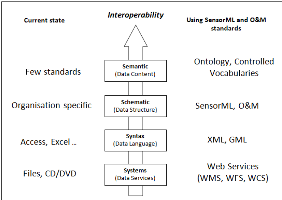
Figure 1. Levels of technical interoperability (according to GeoSciML – modified and complemented)
