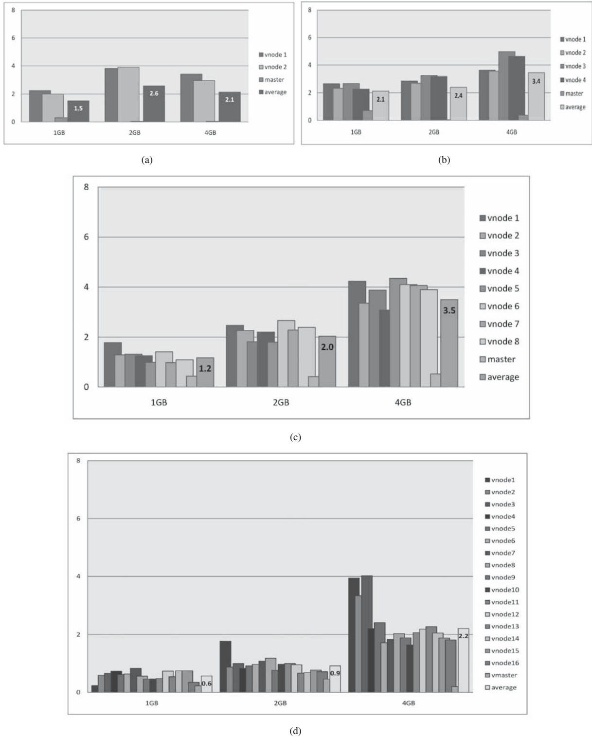
Fig. 4. System load, as measured by the Linux uptime command, for 2(a), 4(b), 8(c), and 16(d) nodes. Note that the master node load, indicated by the penultimate solid bar, in each configuration is well below the average, illustrated by the last hatched bar.
