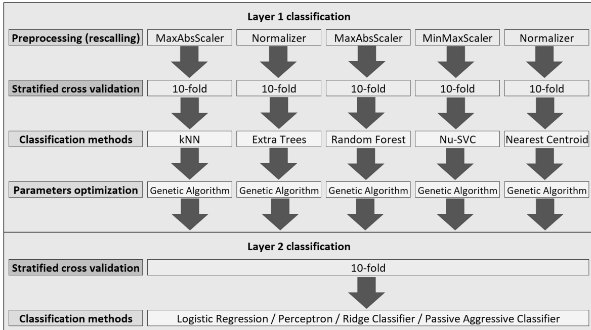
Fig. 7. Flowchart of ML Algorithm 4.
